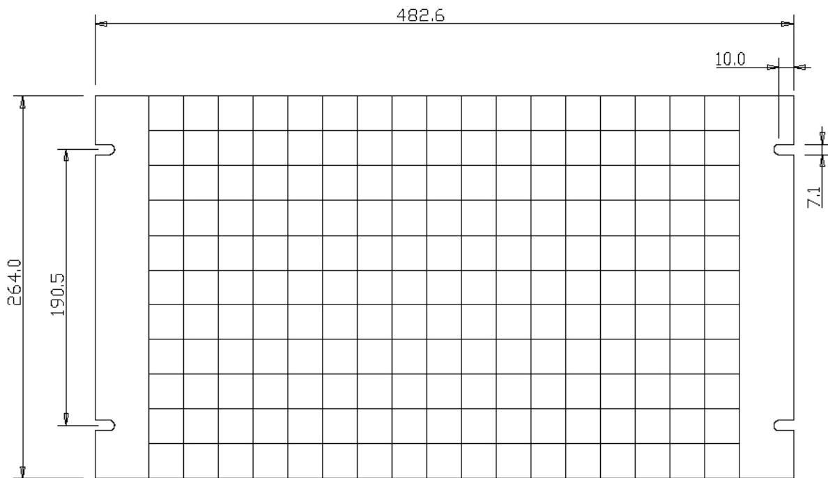
Standard utilising 24 x 24 mm tiles
