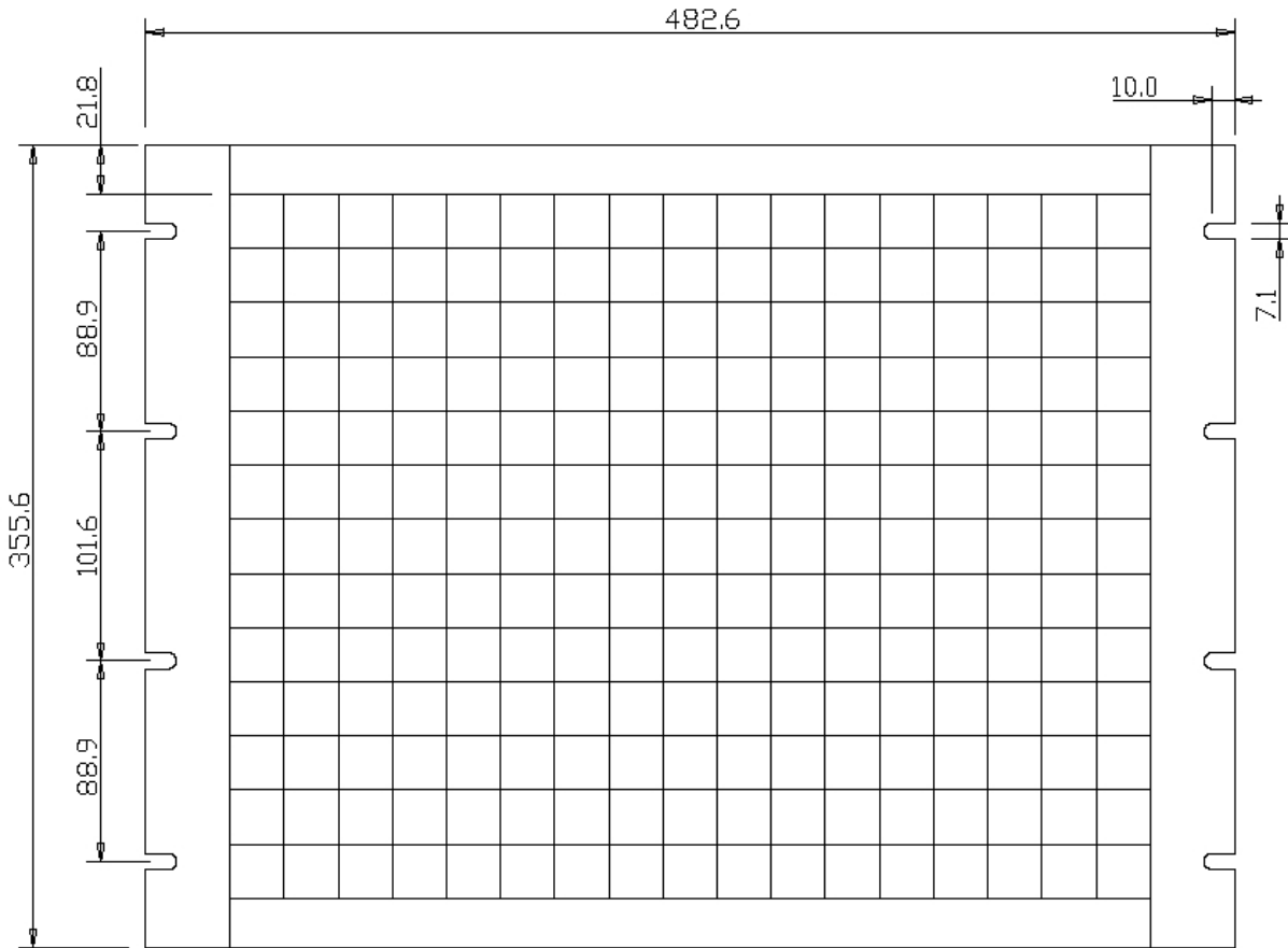
Standard utilising 24 x 24 mm tiles
