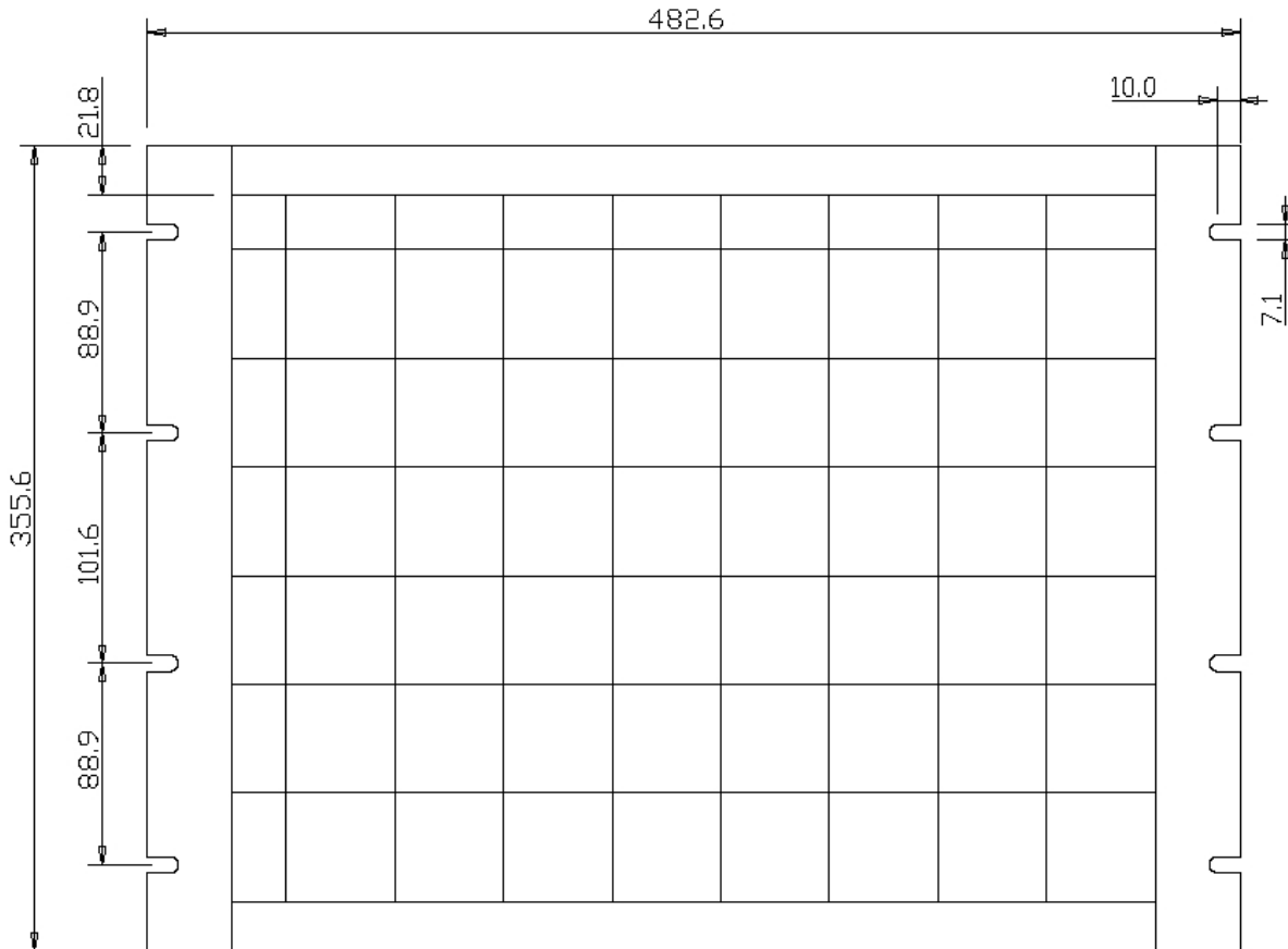
Alternative utilising 24 x 24, 24 x 48 and 48 x 48 mm tiles
