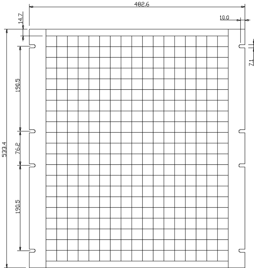
Standard utilising 24 x 24 mm tiles
