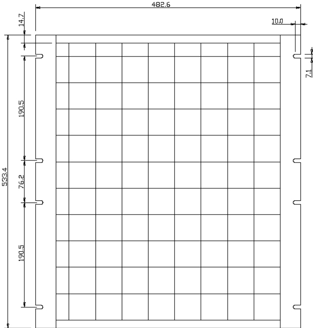
Alternative utilising 24 x 24, 24 x 48 and 48 x 48 mm tiles
