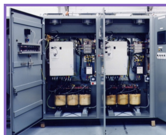
Borehole Extraction VSD Pump Control
